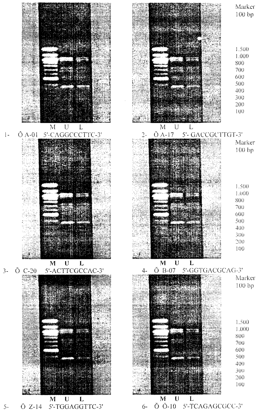
Fig. (3): DNA gel electrophoresis bands using 6 primers
