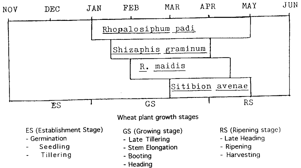
Fig. 1. Seasonal incidence of aphid species throughout different growth stages of the wheat plant in Egypt.
